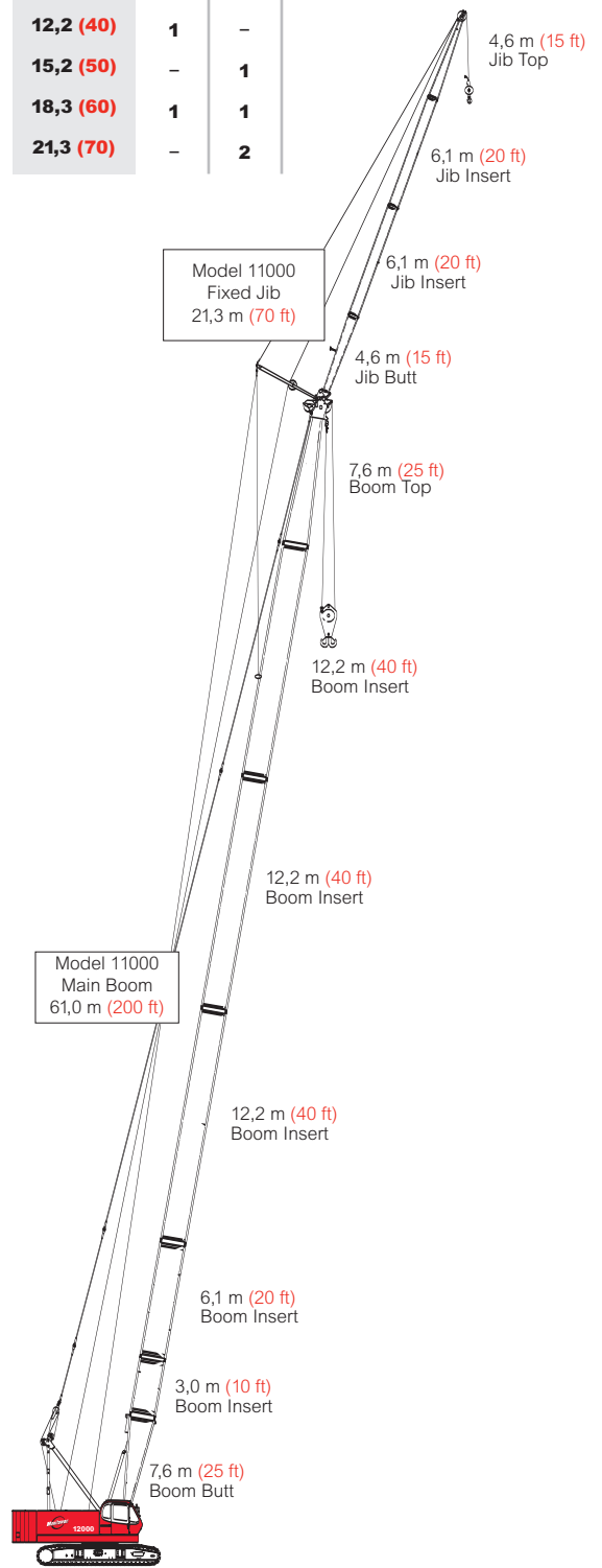
Model 11000 Fixed Jib on Main Boom 82,3 m (270 ft)
