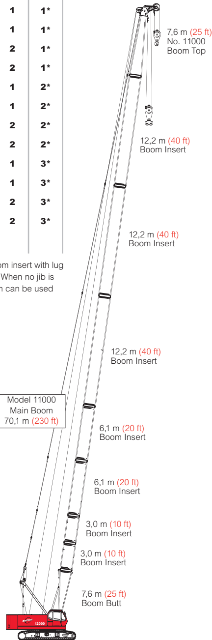
Model 11000 Main Boom 70,1 m (230 ft)
