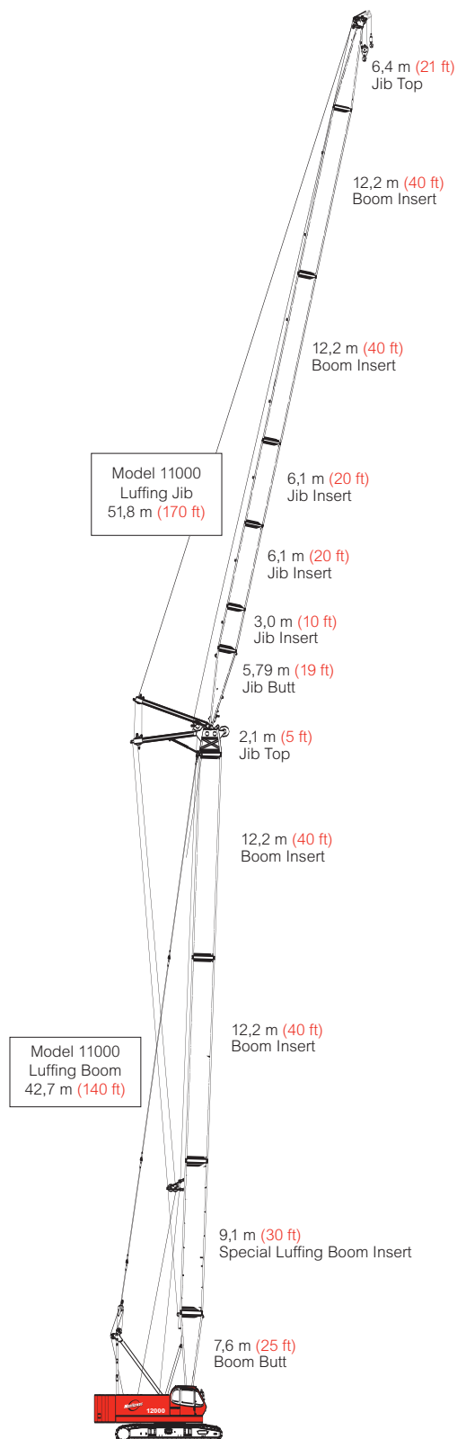
Model 11000 Luffing Jib on Luffing Boom 94,5 m (310 ft)
