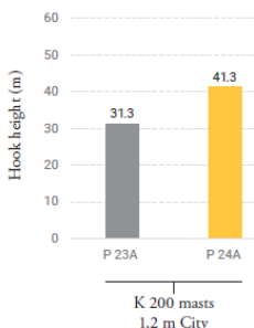
Hook heights MDT159 --> 45 m jib / C50
