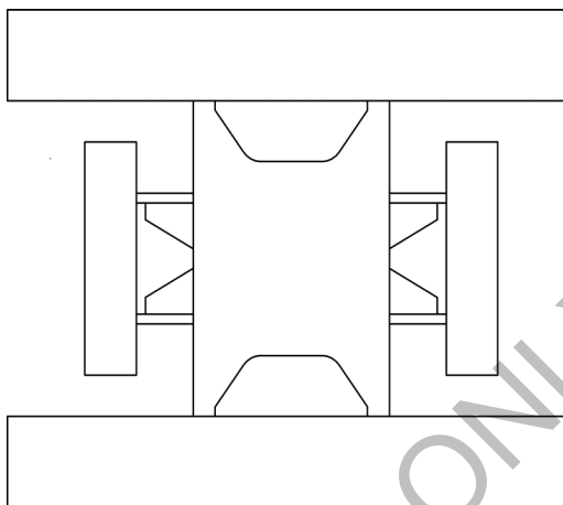
MLC200 SERIES 2 or MLC200 SERIES 3 27 400 kg (60,400 lb) Carbody Counterweight (2 center boxes with platforms)
